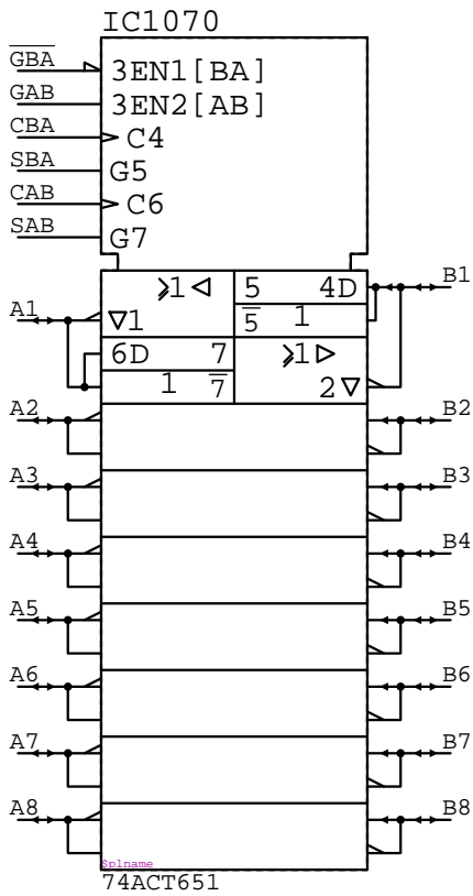
74ACT651 IC?????
