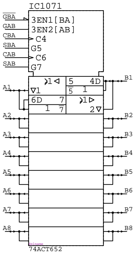
74ACT652 IC?????
