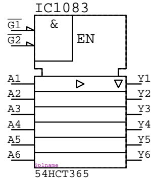
54HCT365 IC?????
