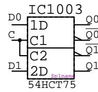
54HCT75 IC????
