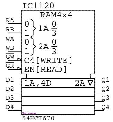
54HCT670 IC?????
