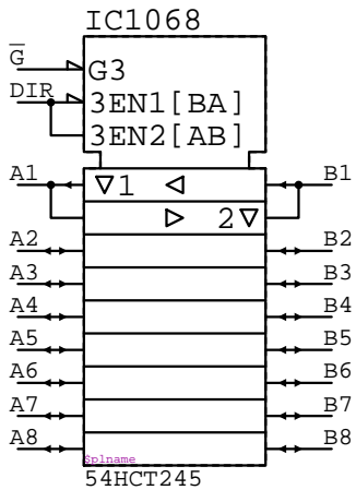
54HCT245 IC????
