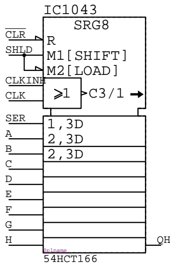
54HCT166 IC????
