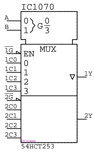
54HCT253 IC????
