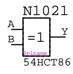
54HCT86 N????
