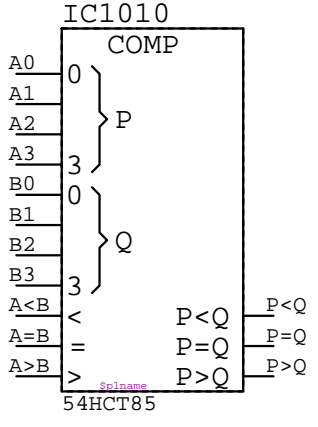
54HCT85 IC????
