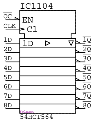
54HCT564 IC????
