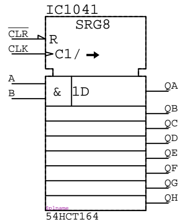
54HCT164 IC????
