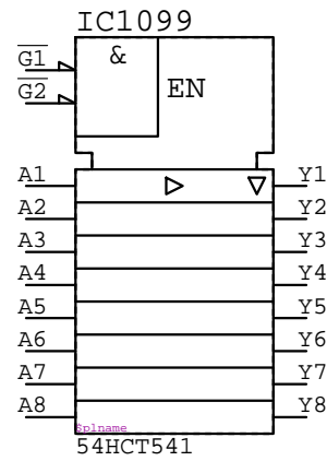
54HCT541 IC????
