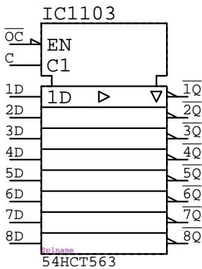
54HCT563 IC????
