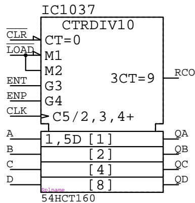
54HCT160 IC????
