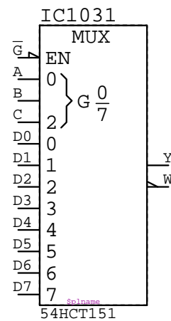
54HCT151 IC????
