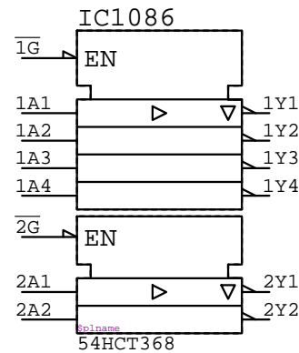
54HCT368 IC?????
