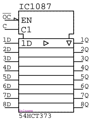
54HCT373 IC?????
