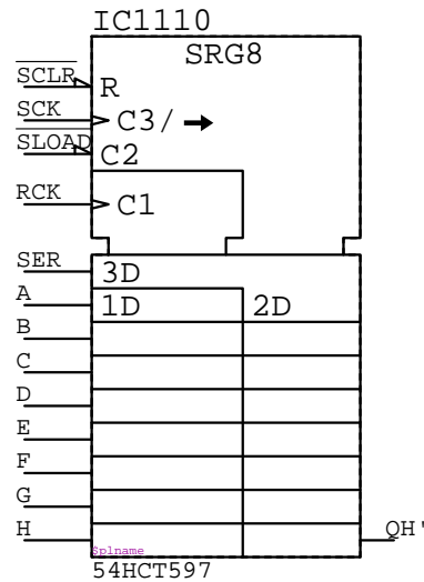
54HCT597 IC????
