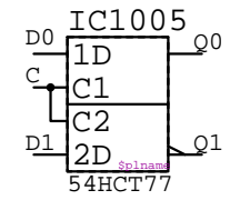
54HCT77 IC????
