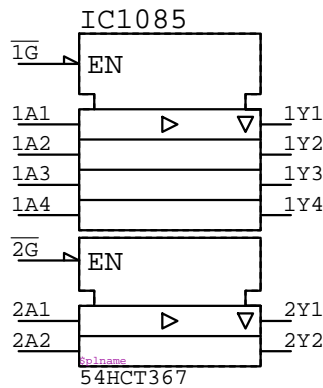
54HCT367 IC?????
