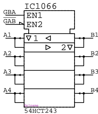
54HCT243 IC?????
