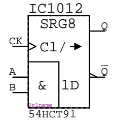
54HCT91 IC????
