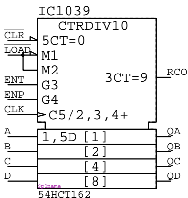
54HCT162 IC????
