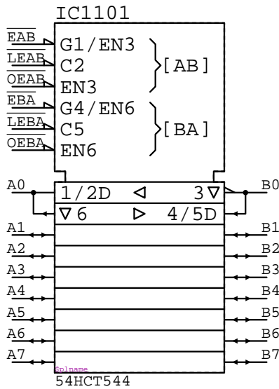
54HCT544 IC????
