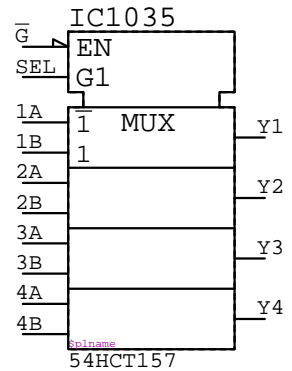
54HCT157 IC????
