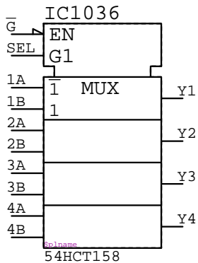
54HCT158 IC????
