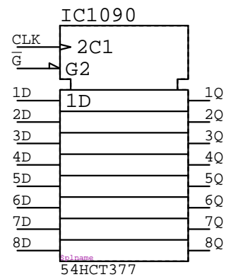
54HCT377 IC?????
