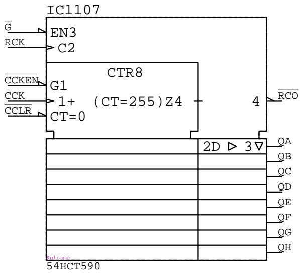
54HCT590 IC????
