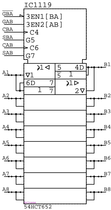
54HCT652 IC?????
