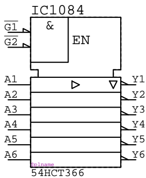
54HCT366 IC?????
