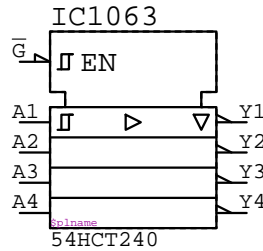
54HCT240 IC?????
