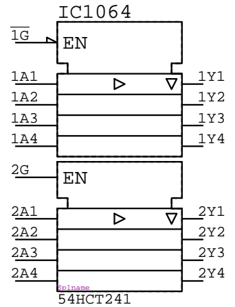
54HCT241 IC?????
