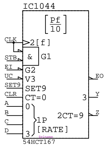
54HCT167 IC????
