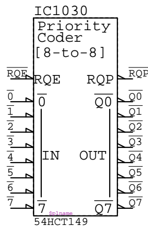
54HCT149 IC????
