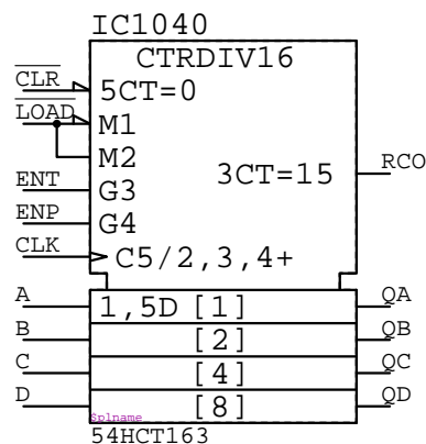
54HCT163 IC????
