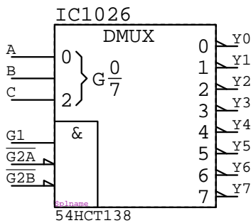
54HCT138 IC????
