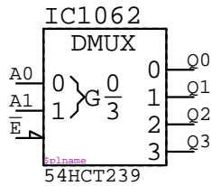
54HCT239 IC?????
