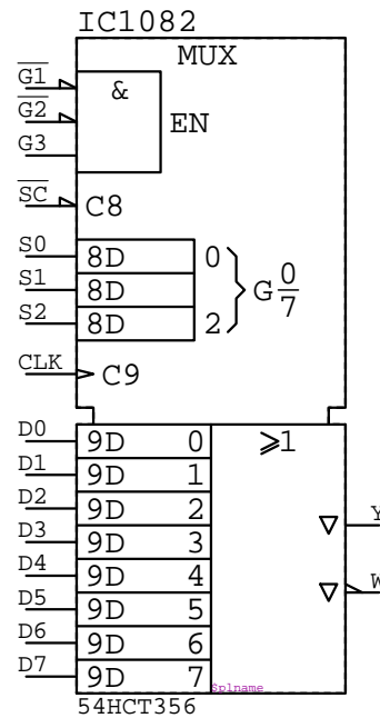
54HCT356 IC?????
