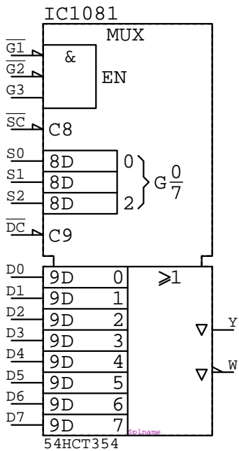
54HCT354 IC?????
