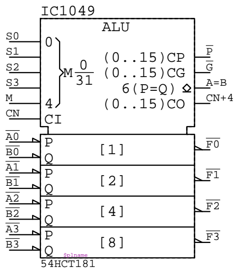
54HCT181 IC????
