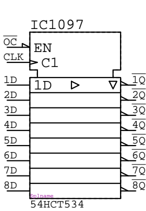
54HCT534 IC????
