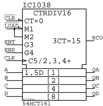
54HCT161 IC????
