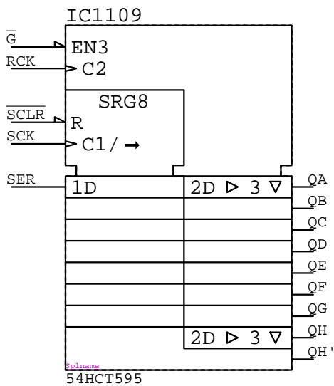
54HCT595 IC????
