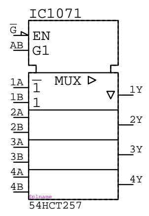
54HCT257 IC????
