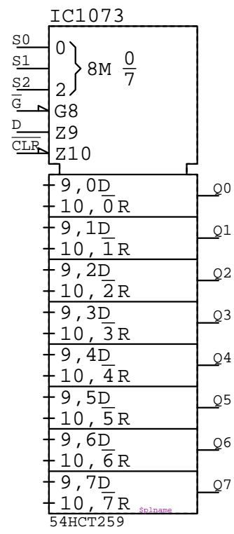
54HCT259 IC????
