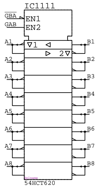
54HCT620 IC????
