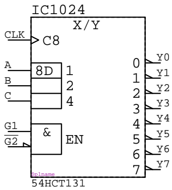
54HCT131 IC????
