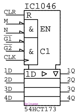
54HCT173 IC????
