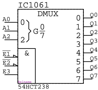
54HCT238 IC?????
