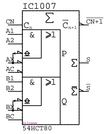
54HCT80 IC????
