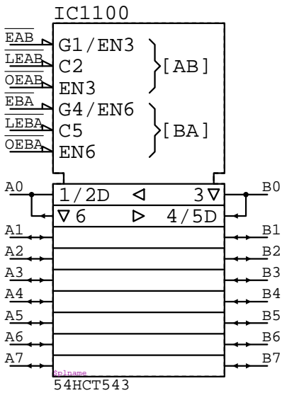
54HCT543 IC????
