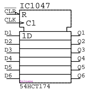
54HCT174 IC????
