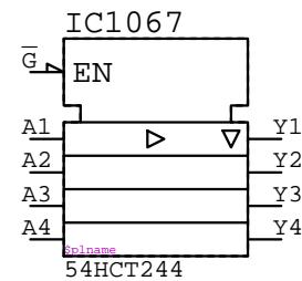
54HCT244 IC?????
