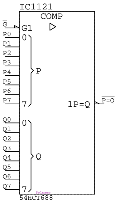
54HCT688 IC?????
