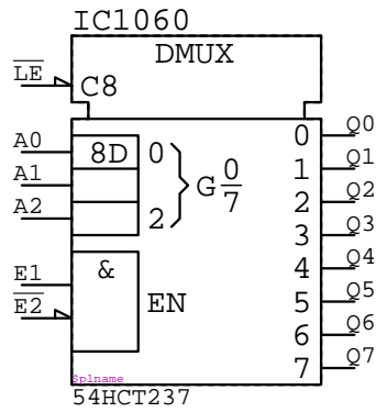
54HCT237 IC?????
