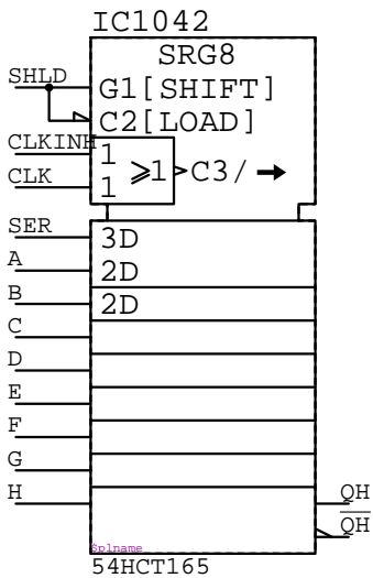
54HCT165 IC????
