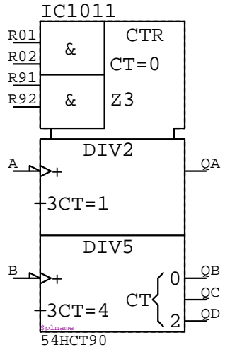
54HCT90 IC????
