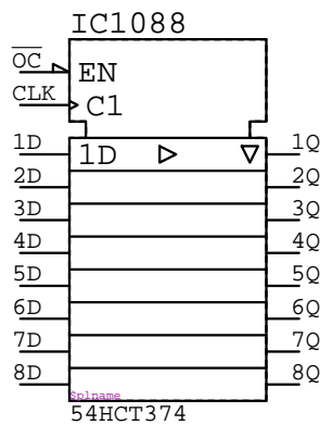
54HCT374 IC?????
