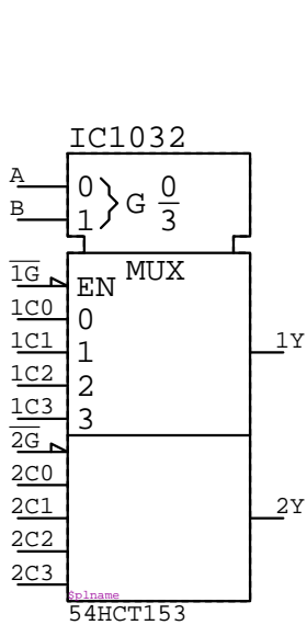
54HCT153 IC????
