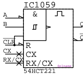
54HCT221 IC?????
