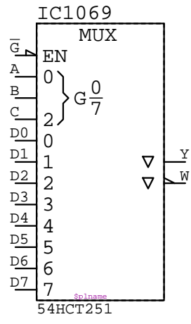
54HCT251 IC????
