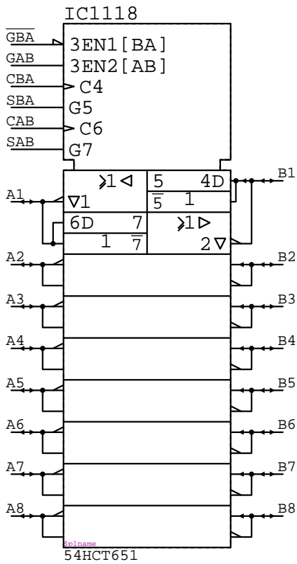
54HCT651 IC?????
