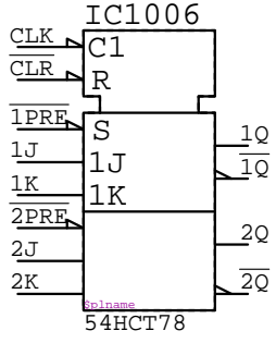
54HCT78 IC????
