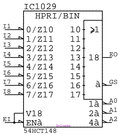
54HCT148 IC????
