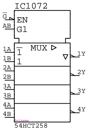
54HCT258 IC????
