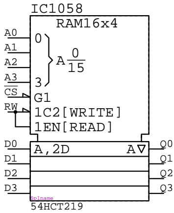
54HCT219 IC?????
