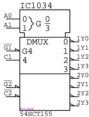
54HCT155 IC????
