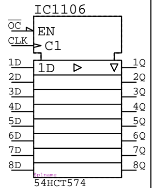
54HCT574 IC????
