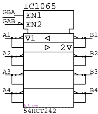
54HCT242 IC?????
