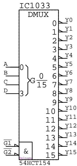
54HCT154 IC????
