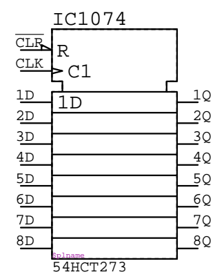
54HCT273 IC????
