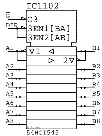
54HCT545 IC????
