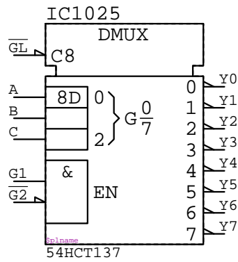
54HCT137 IC????
