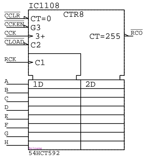
54HCT592 IC????
