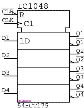
54HCT175 IC????
