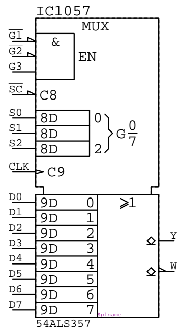
54ALS357 IC????
