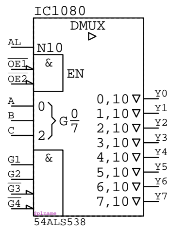
54ALS538 IC????
