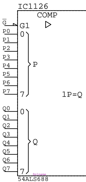
54ALS688 IC????
