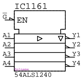
54ALS1240 IC????
