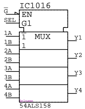
54ALS158 IC????
