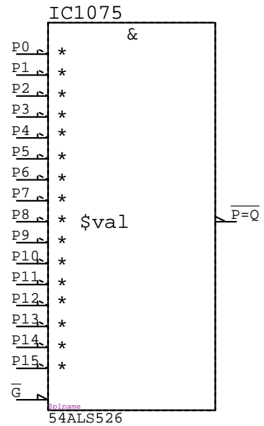
54ALS526 IC?????
