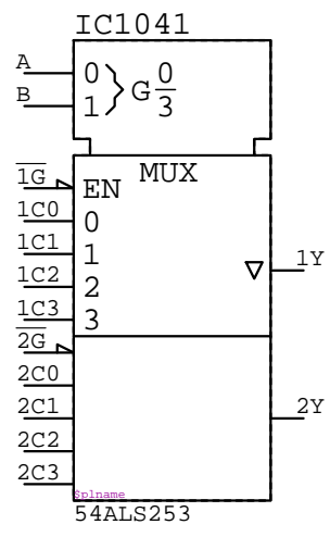
54ALS253 IC????
