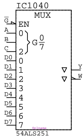
54ALS251 IC????
