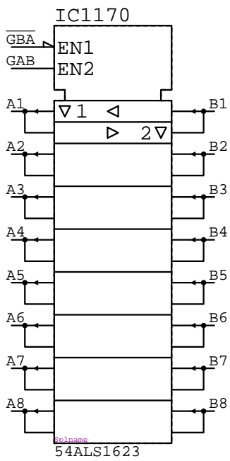
54ALS1623 IC????
