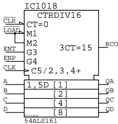
54ALS161 IC????
