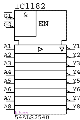
54ALS2540 IC????
