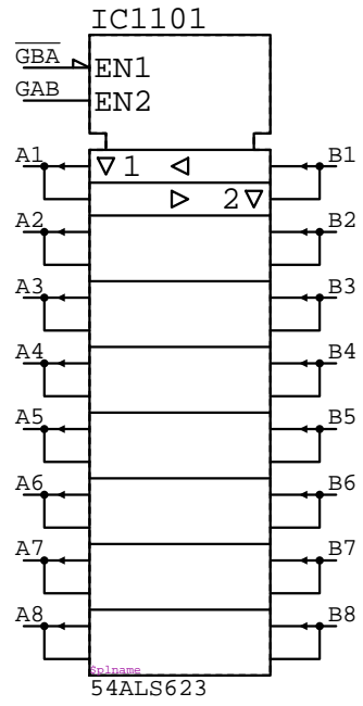
54ALS623 IC????
