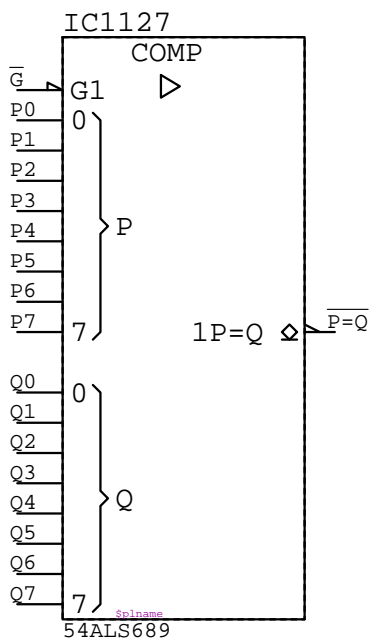
54ALS689 IC????
