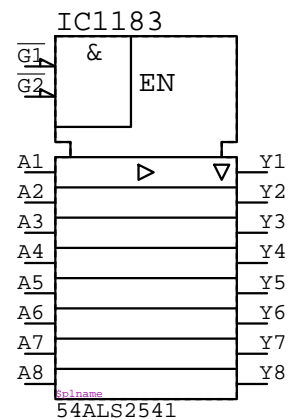
54ALS2541 IC????
