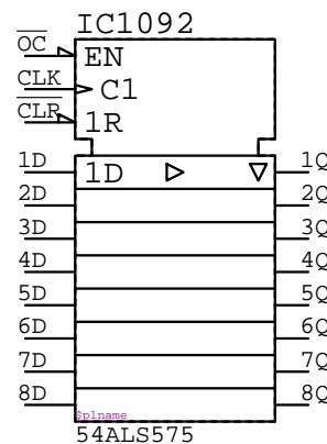
54ALS575 IC?????
