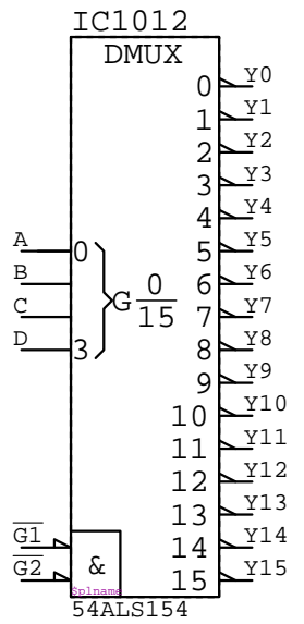
54ALS154 IC????
