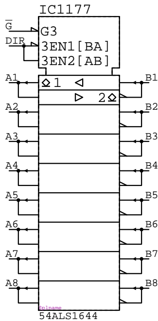
54ALS1644 IC????
