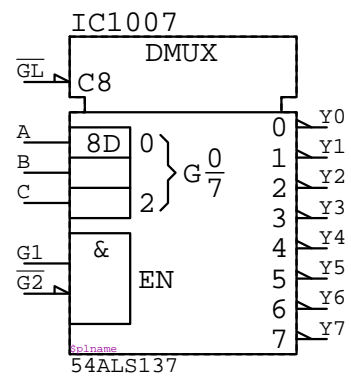
54ALS137 IC????
