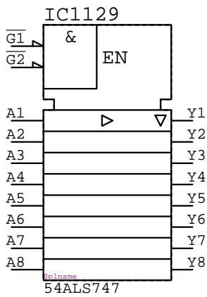
54ALS747 IC????
