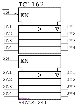
54ALS1241 IC????
