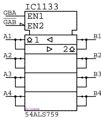
54ALS759 IC????
