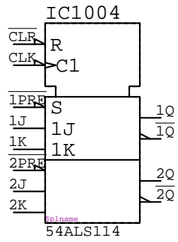
54ALS114 IC????
