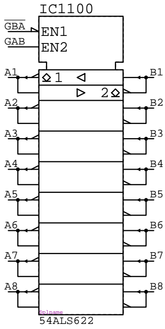
54ALS622 IC????
