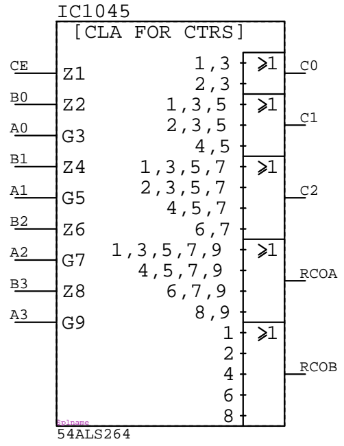
54ALS264 IC????
