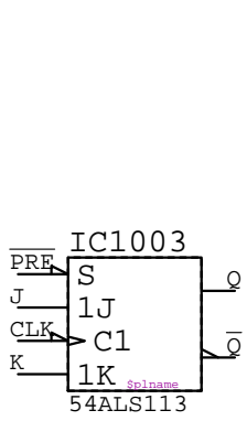
54ALS113 IC????
