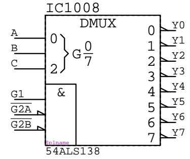
54ALS138 IC????
