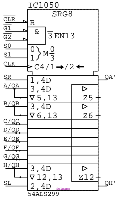
54ALS299 IC????
