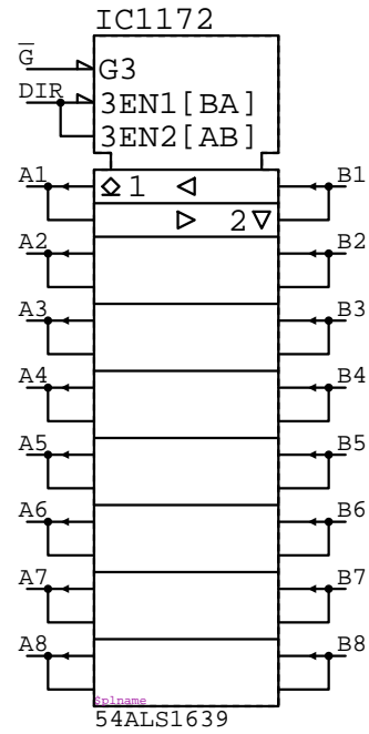
54ALS1639 IC????
