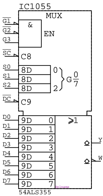
54ALS355 IC????
