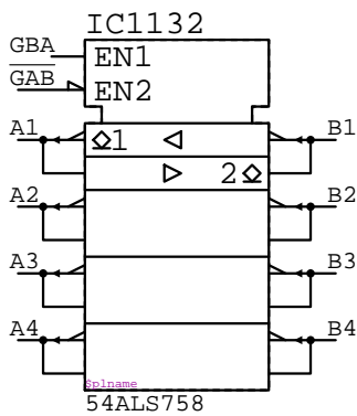
54ALS758 IC????
