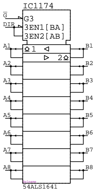
54ALS1641 IC????
