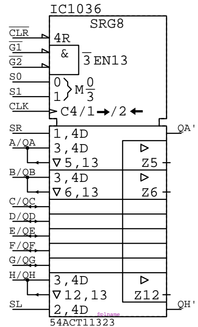
54ACT11323 IC????
