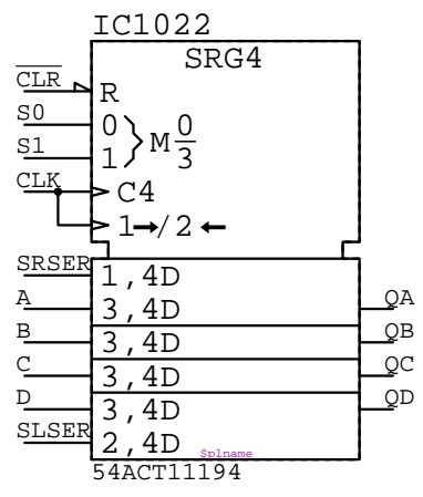
54ACT11194 IC?????
