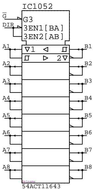
54ACT11643 IC????
