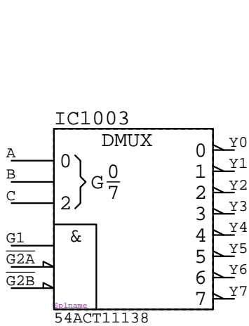
54ACT11138 IC?????
