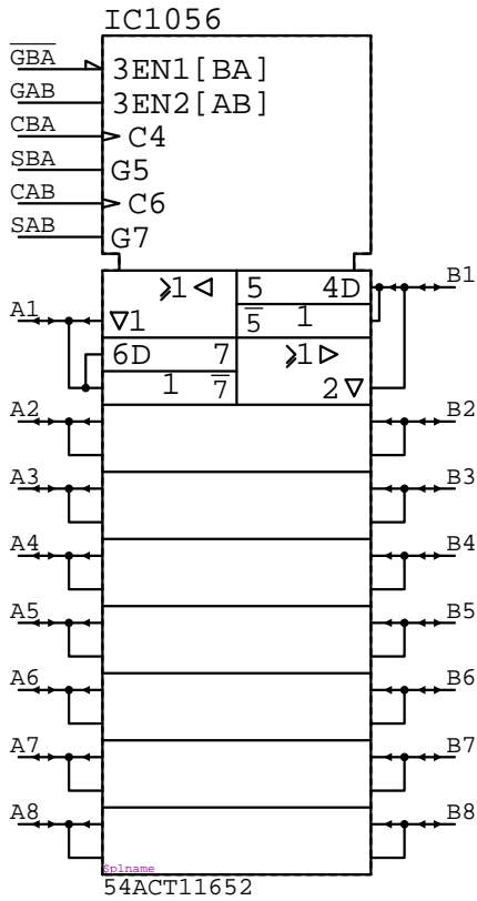
54ACT11652 IC?????
