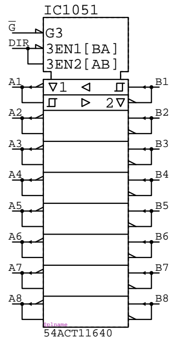
54ACT11640 IC????
