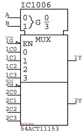
54ACT11153 IC?????
