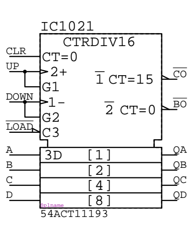
54ACT11193 IC?????
