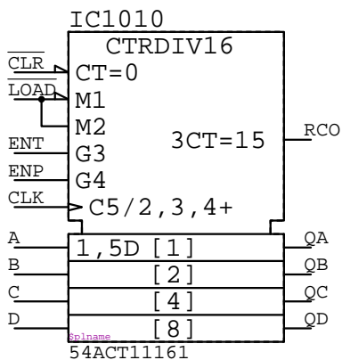
54ACT11161 IC?????
