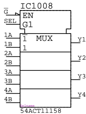
54ACT11158 IC?????
