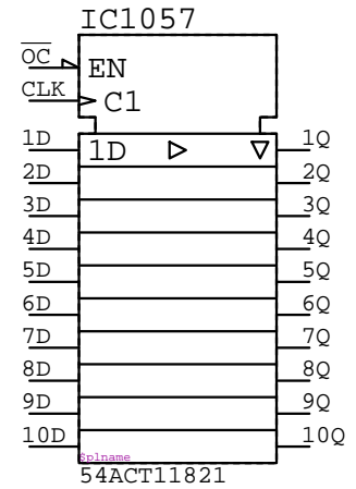
54ACT11821 IC?????
