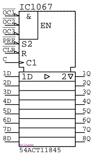
54ACT11845 IC????
