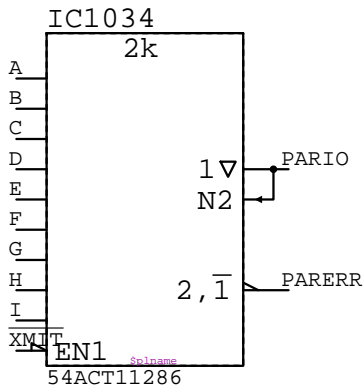
54ACT11286 IC????
