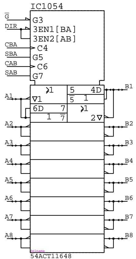
54ACT11648 IC????
