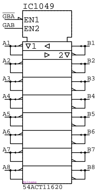
54ACT11620 IC????
