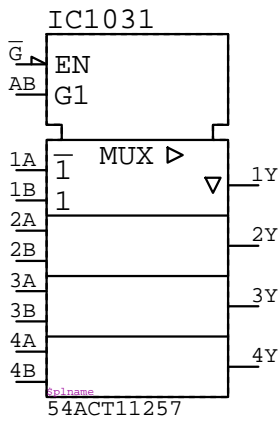
54ACT11257 IC????
