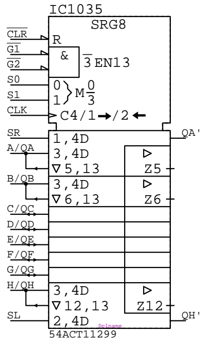
54ACT11299 IC????
