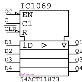
54ACT11873 IC????
