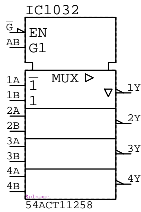
54ACT11258 IC????
