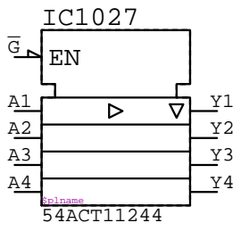
54ACT11244 IC?????
