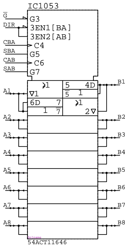
54ACT11646 IC????
