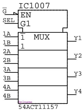
54ACT11157 IC?????
