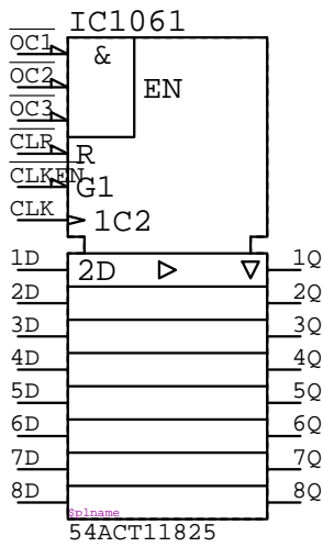
54ACT11825 IC????
