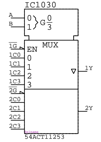
54ACT11253 IC?????
