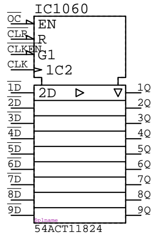
54ACT11824 IC?????
