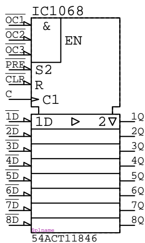
54ACT11846 IC????
