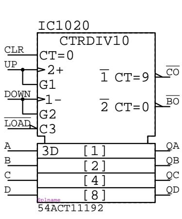
54ACT11192 IC?????
