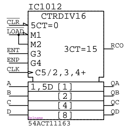
54ACT11163 IC?????
