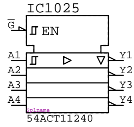
54ACT11240 IC?????
