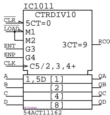
54ACT11162 IC?????
