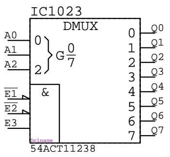
54ACT11238 IC?????
