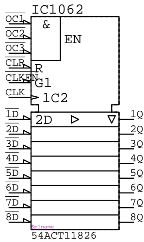
54ACT11826 IC????
