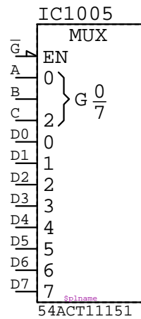
54ACT11151 IC?????
