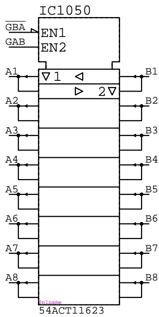
54ACT11623 IC????
